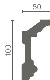
DD503 — 100x50x2000 MM
