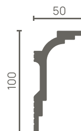
DD515 — 100x50x2000 MM
